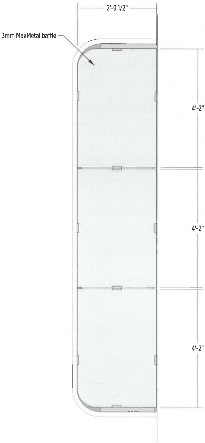
2 DETAIL @ Internal LED Baffle 02.02 Scale: 1/2"=1'-0"
