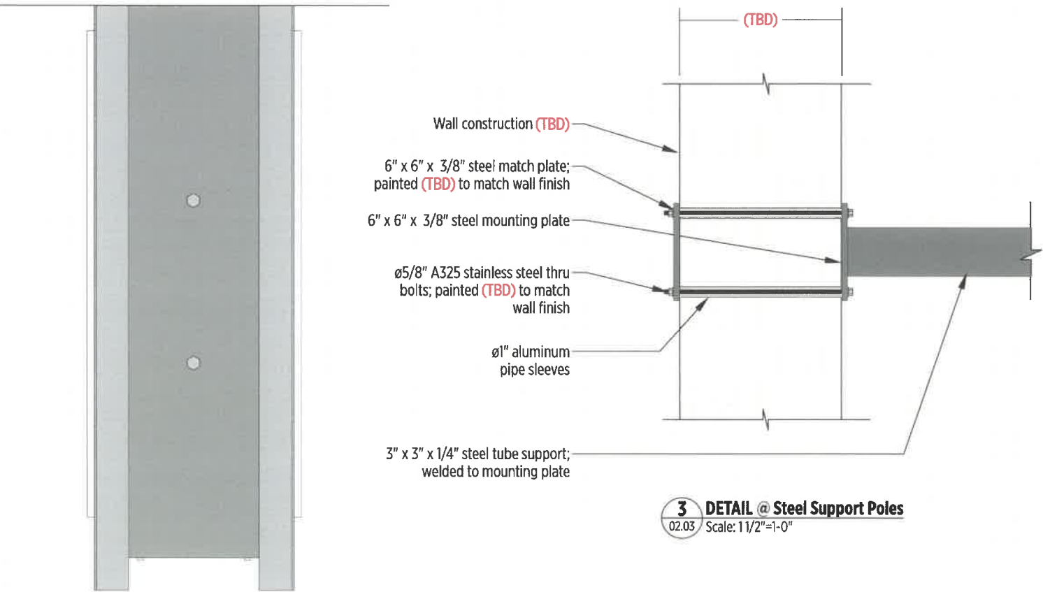
2 FRAMING DETAIL 02.03 Scale: 1-1/2"=1'-0"
