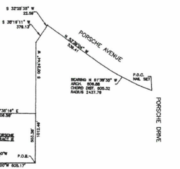
POINT OF COMMENCEMENT TO POINT OF BEGINNING N.T.S.
